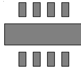
Figure 10 (c). Copper Area = 30mm 2 , θ JA = 54°C/W
