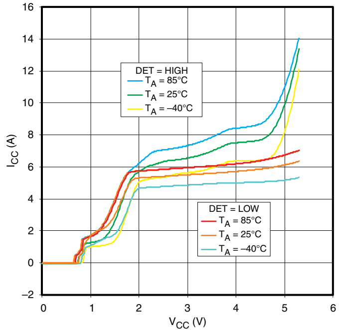
Figure 2. I CC vs V CC , EN = V CC
