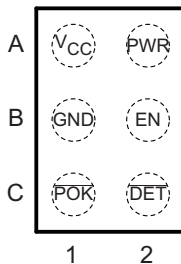
YFP PACKAGE (TOP-THROUGH VIEW)
