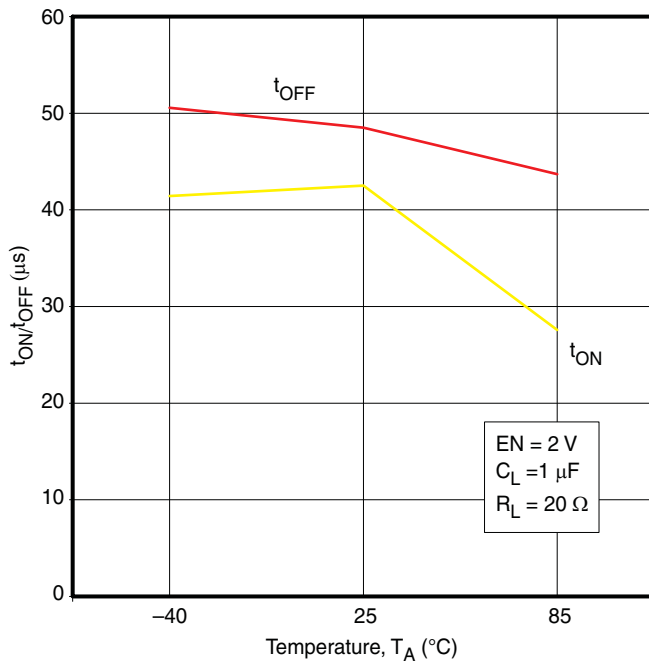
Figure 5. t_{ON}/t_{OFF} vs Temperature, V_{CC} = 5.3 V
