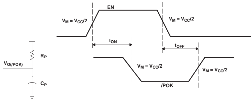
Figure 11. EN to POK Test Point
