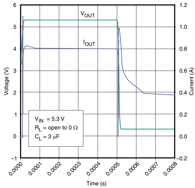
Figure 9. No Load to Short-Circuit Transient Response
