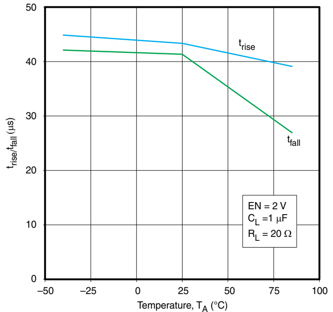
Figure 4. t rise /t fall vs Temperature, V CC = 5.3 V
