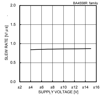
Slew Rate - Supply Voltage ( C_L=100[pF] , R_L=2[k\Omega] , T_a=25[°C] )
