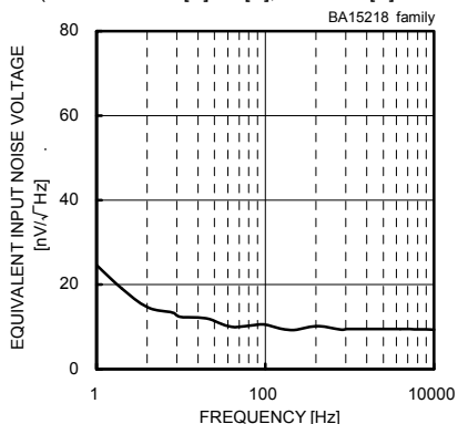
Fig. 217 Equivalent Input Noise Voltage - Frequency (VCC/VEE=+15[V]/-15[V], Rs=100[Ω], Ta=25[°C])
