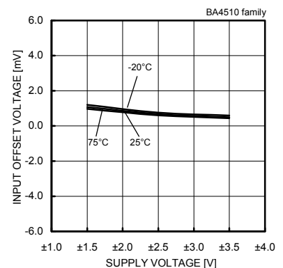
Fig. 273 Input Offset Voltage - Supply Voltage (V icm =0[V], V out =0[V])
