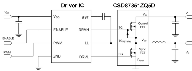
TYPICAL CIRCUIT
