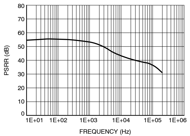
Figure 12. PSRR @ 10 mA
