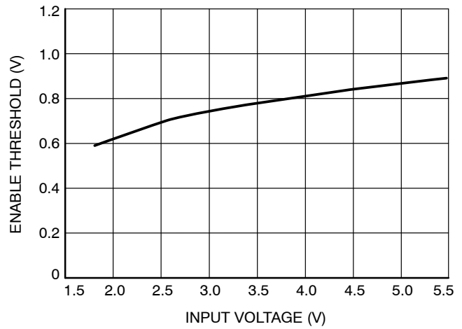
Figure 10. Falling Enable Threshold vs. Supply Voltage
