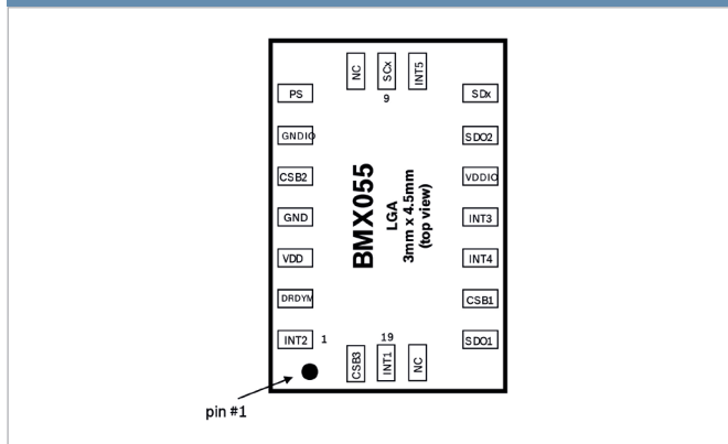
Pin configuration (top view, pads not visible)
