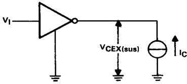
FIGURE 1. V_{CEX(sus)}
