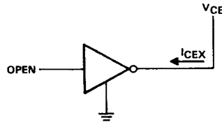
FIGURE 2. I_{CEX}
