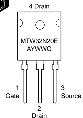
TO-247AE CASE 340K STYLE 1
