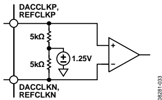
Figure 61. Clock Receiver Input Equivalent Circuit
